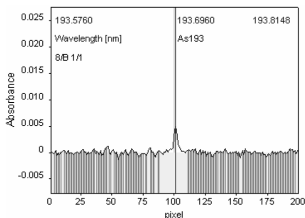
Figure 1. Linear spectrum of a rainbow trout
