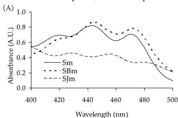
Figure 1. UV-Vis spectra of oil extracts (dilution 1:100), useful to identify their specific fingerprint for 2 classes of bioactive molecules: (A) carotenoids ( \lambda_{\text{max}} : 420–480 nm) and (B) polyphenols ( \lambda_{\text{max}} : 260–280 and 350–360 nm)
