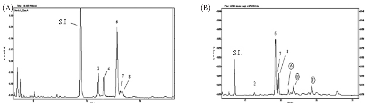
Figure 3. GC-FID fingerprint of esterified sterols useful to discriminate between soybean oil (SO) (A), seabuckthorn oil (SBO) (B). Peak identification: S.I.: 5 \alpha -colestan-3 \beta -ol; 2: campesterol; 4: Stigmasterol; 6: \beta -sitosterol; 7: sitostanol; 8: \Delta^5 -avenasterol; A and X – unidentified sterols
