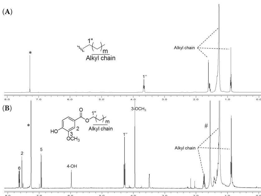
Figure 2. ^1\text{H} NMR spectra of PLs (A) and policosanyl vanillate (B) *solvent peak ( \text{CDCl}_3 ); #water peak
