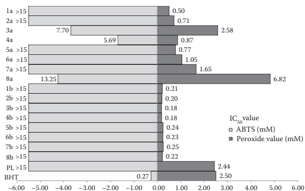
Figure 3. Concentration of antioxidant necessary to reduce oxidation by 50%, determined using ABTS and FTC assays
