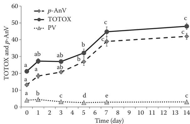
Figure 4. Oxidation trend of linoleic acid. Different letters in one line show significant differences ( P < 0.05 )
