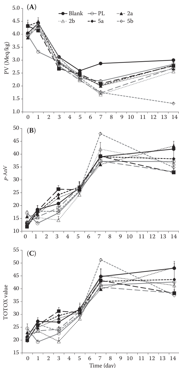
Figure 6. Inhibitory effect on PV (A), p -AnV (B), and TOTOX (C) in a linoleic acid model system (sample concentrations are 100 \mu M)
