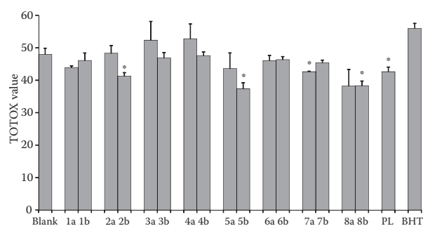
Figure 5. Inhibitory effect on the TOTOX value at 14 days *means significantly lower than the blank, P < 0.05 ; sample concentrations are 100 \mu M
