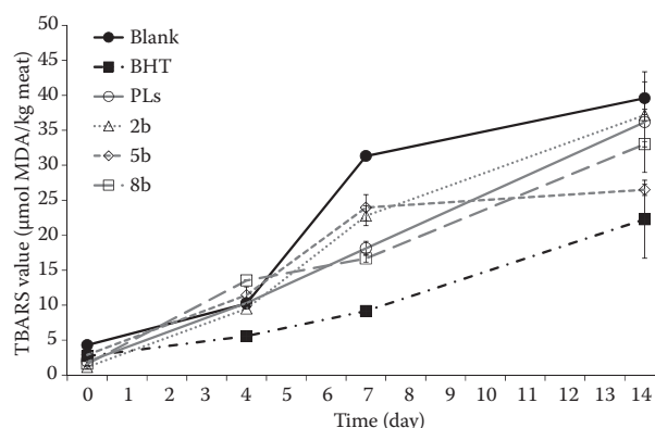
Figure 7. Thiobarbituric acid reactive substance (TBARS) values in cooked pork (sample concentrations are 100 \mu M)
