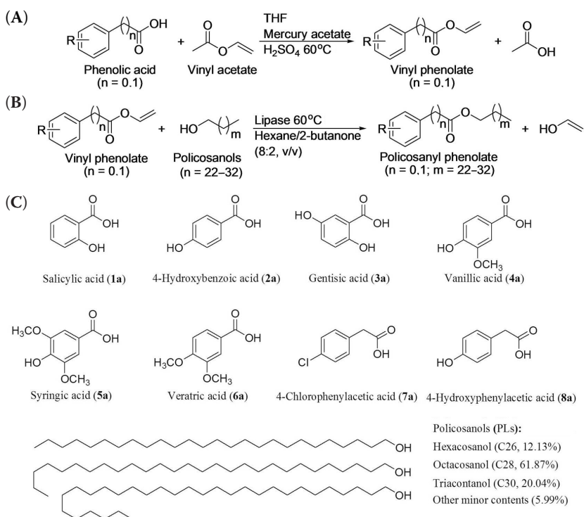
Figure 1. Scheme for policosanyl phenolate synthesis: (A) chemical vinylation; (B) lipase-catalysed esterification; (C) structures of policosanols and phenolic acids.
