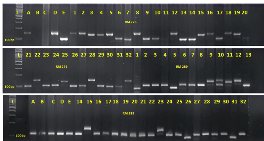
Figure 5. Screening of rice landrace using SSR markers using drought linked QTL SSR markers
