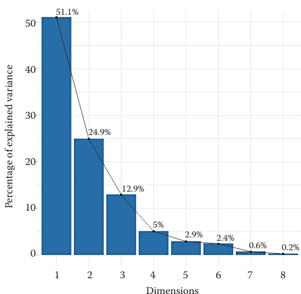
Figure 2. Scree plot diagram based on principal components of 37 rice landraces
