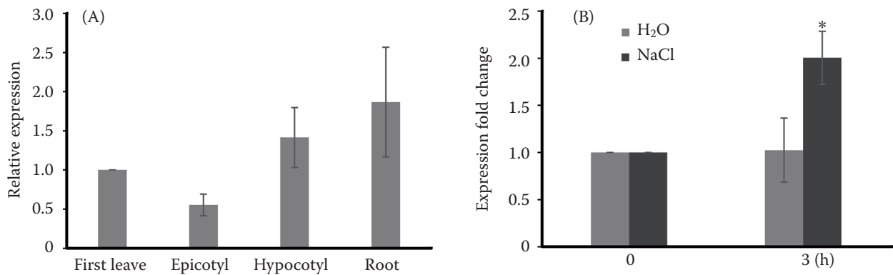
Figure 2. Expression analysis of VuCERK1 : Expression of VuCERK1 in different tissues of cowpea seedling (A); induced expression of VuCERK1 by NaCl treatment in cowpea root (B)
