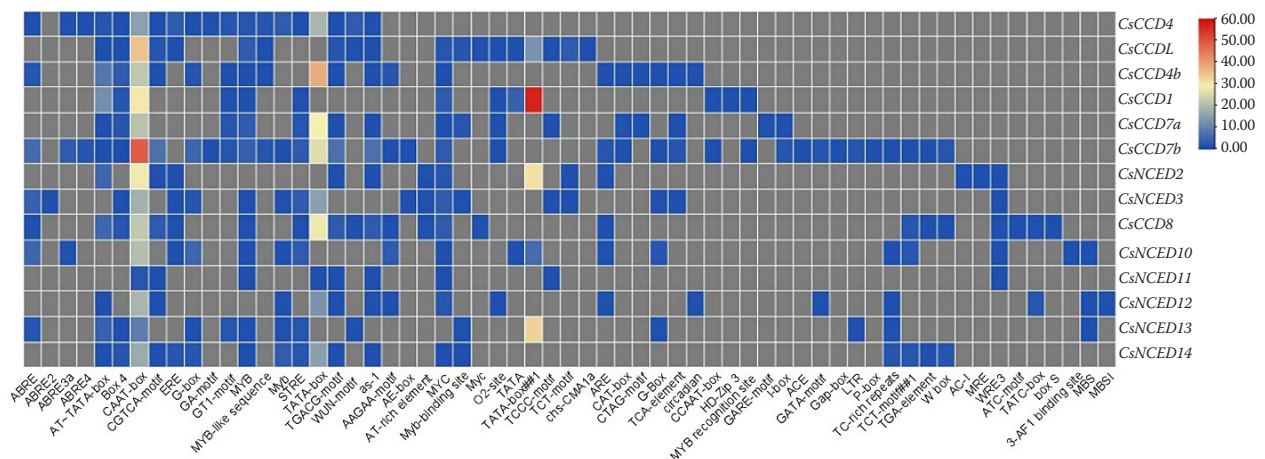
Figure 7. Cis-acting regulatory elements analysis (CAREs) of growth and development, light, hormones, temperature, defence and drought responsive associated elements of 1 000 bp promoter sequences of CCO genes
