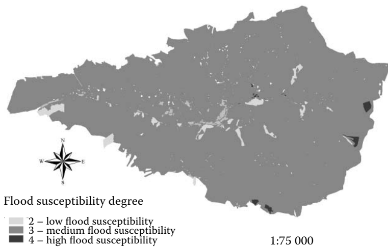
Fig. 1. The Hucava catchment susceptibility to floods
