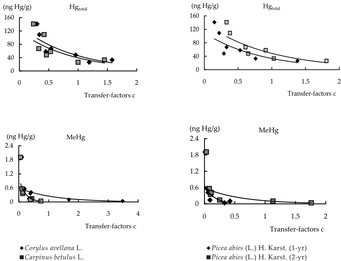
Figure 2. Converting course of transfer-factors ( y = a \cdot e^{-bx} ) in relation to the Hg_{total} and MeHg concentrations in soils (transect Žiar); c – related to root zone (10–30 cm deep)
