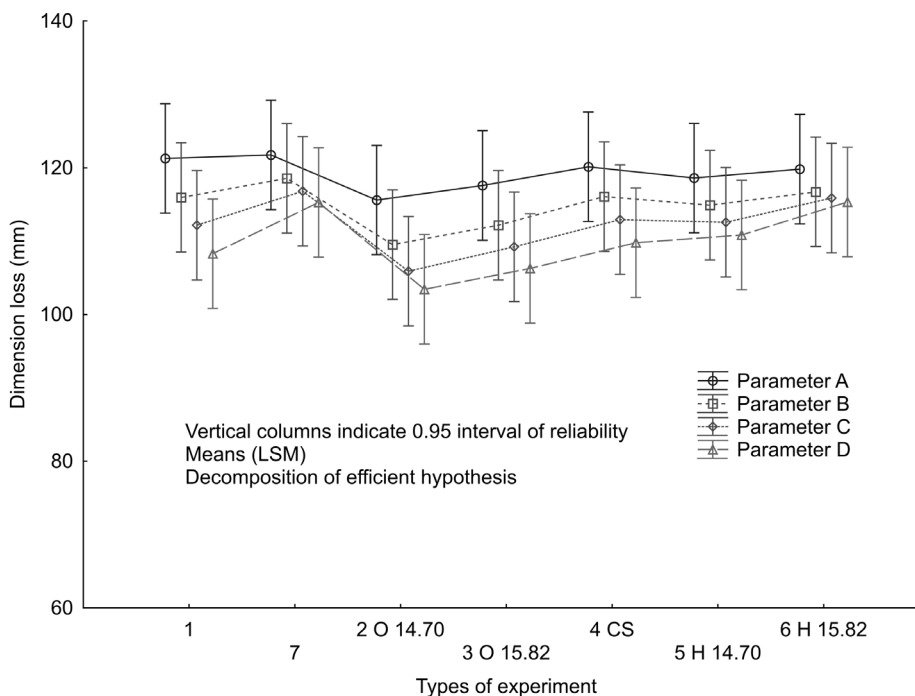
Fig. 3. Change of edge height depending on variant of experiment O – oblique, CS – comparing standard, H – horizontal
