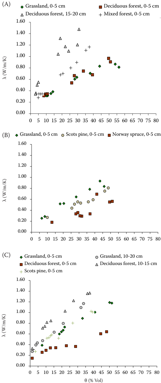
Figure 3. Measured thermal conductivity ( \lambda ) as a function of the soil water content ( \theta ) under different land use in Gabra (A), Govedartsi (B) and Igralishte (C)
