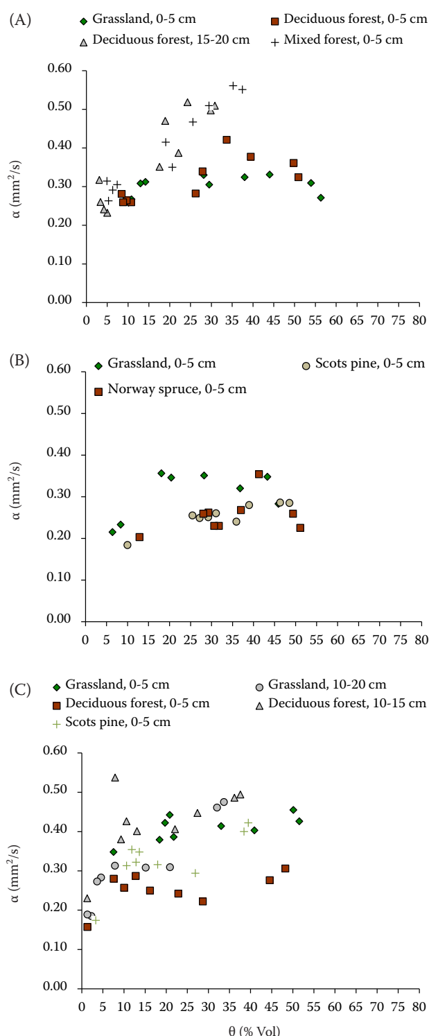
Figure 5. Measured thermal diffusivity ( \alpha ) as a function of the soil water content ( \theta ) under different land use in Gabra (A), Govedartsi (B) and Igralishte (C)
