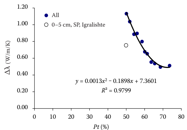
Figure 6. Variation (max-min) of the thermal conductivity ( \Delta\lambda ) observed over the whole range of wetness versus the total porosity ( P_t )
