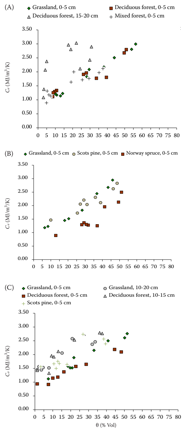
Figure 4. Measured volumetric heat capacity ( C_v ) as a function of the soil water content ( \theta ) under different land use in Gabra (A), Govedartsi (B) and Igralishte (C)
