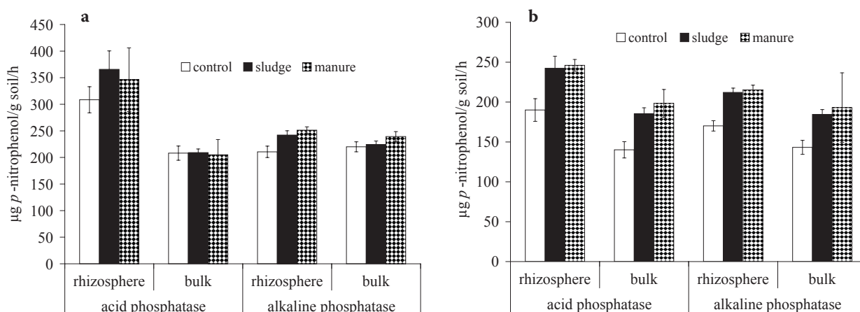
Figure 3. The phosphatase activity in (a) oilseed rape and (b) wheat rhizosphere ( \mu\text{g } p\text{-nitrophenol per 1 g of soil per hour} )
