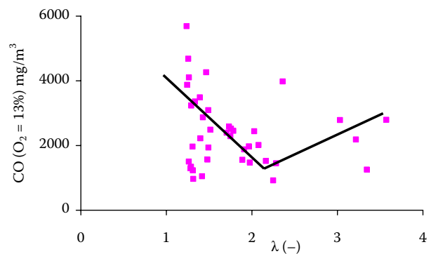
Figure 7. Dependence of CO emissions on excess air factor \lambda at combustion of briquette timothy grass hay
