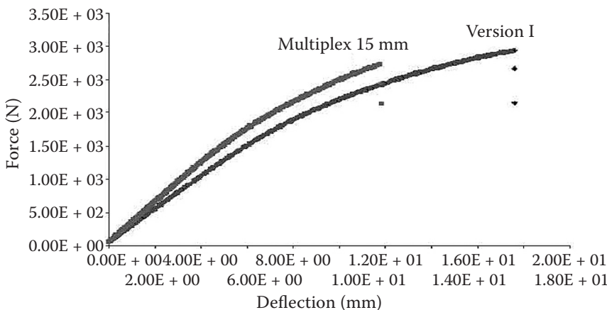
Fig. 7. Comparison of the course of force and deflection – bending strength along the grain – Variant 1
