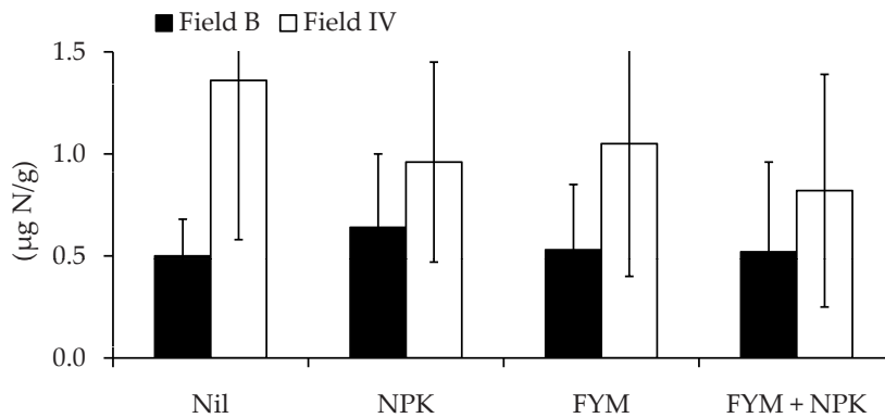
Figure 5. Average values of ammonia nitrogen content (N-NH 4 ) in soil samples from the selected variants of the long-term field experiment in Prague-Ruzyně over the period 1999–2004 (µg N/g)
