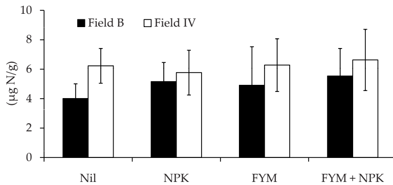
Figure 6. Average values of nitrate nitrogen (N-NO 3 ) content in soil samples from the selected variants of the long-term field experiment in Prague-Ruzyně over the period 1999–2004 (µg N/g)
