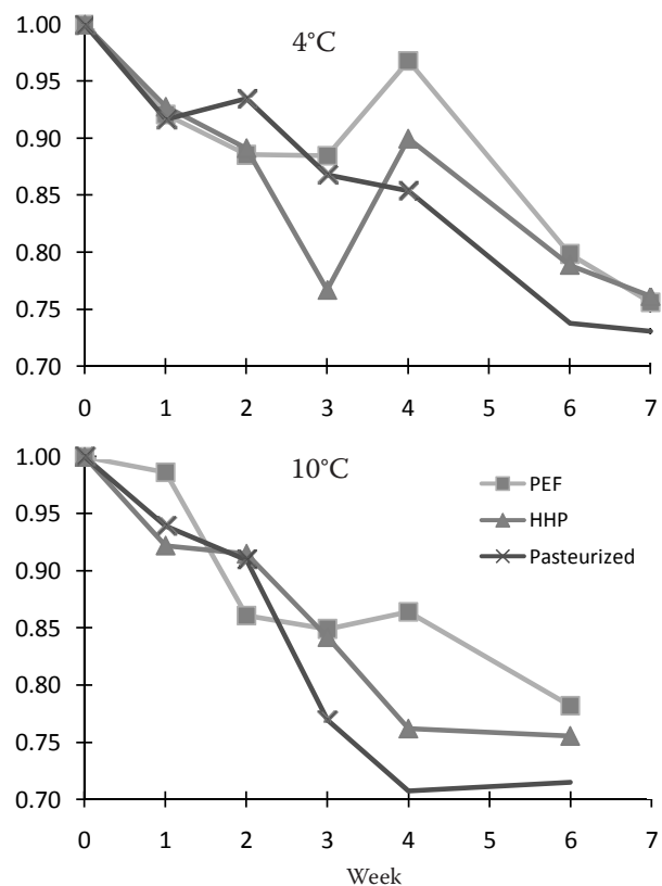
Figure 1. Carotenoids ( C/C_0 ) in PEF, HHP and pasteurised orange juice, during refrigerated storage (4 and 10°C)
