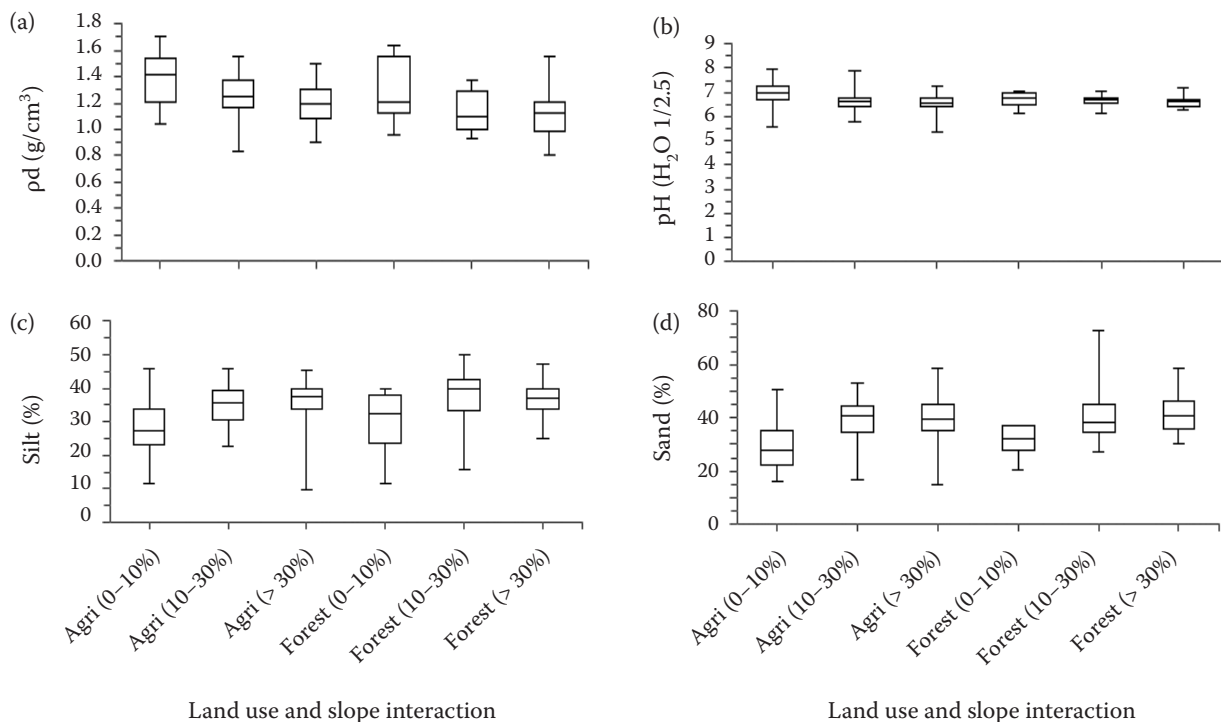
Figure 3. Distribution (box plots with 25 th , mean, and 75 th percentile) across the different land uses and slope steepness classes: bulk density ( \rho_d , g/cm 3 ) (a), pH (b), silt (%) (c) and sand (%) (d)
