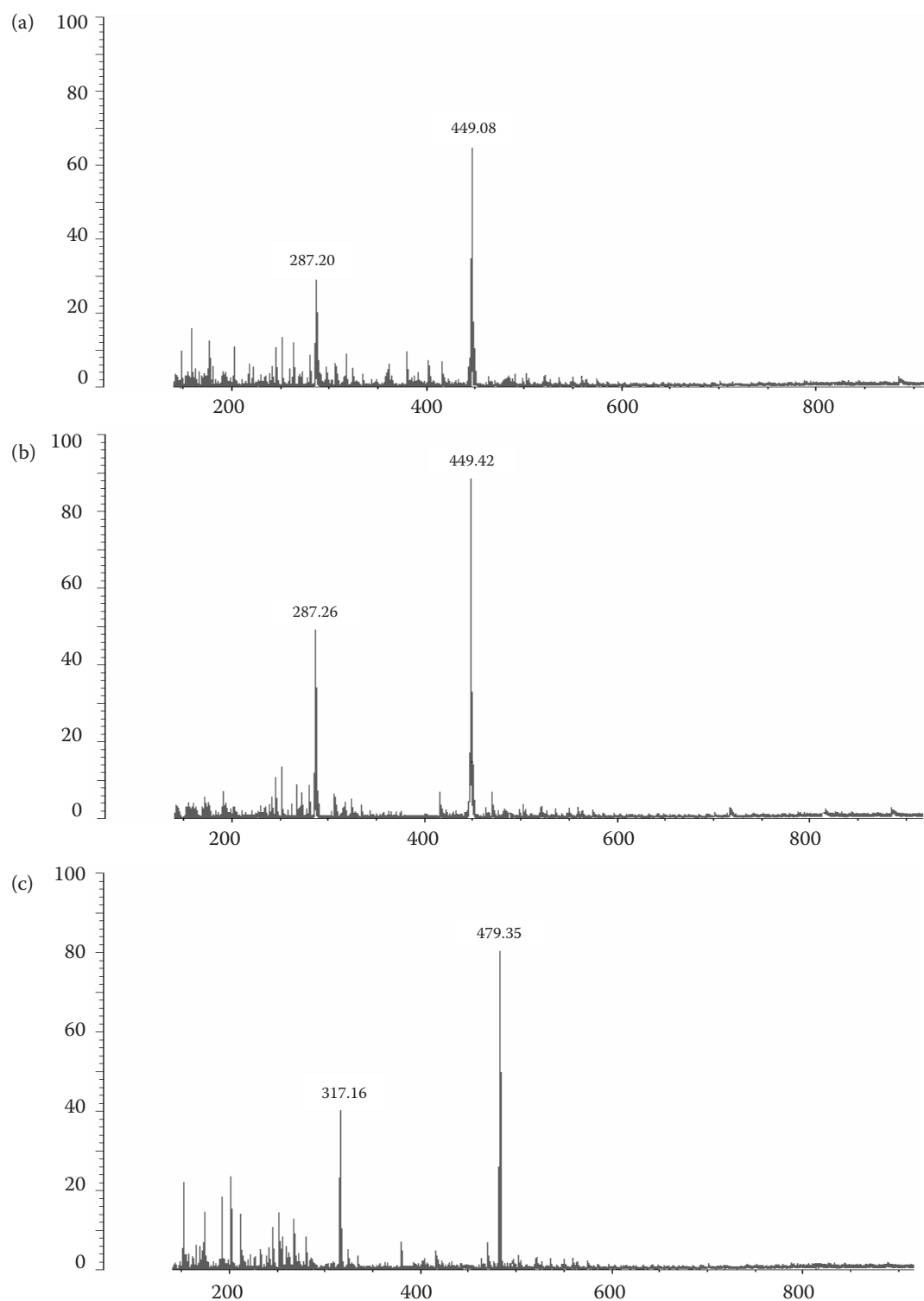
Figure 4. MALDI-TOF-MS of peaks 1–3: (a) peak 1; (b) peak 2; (c) peak 3
