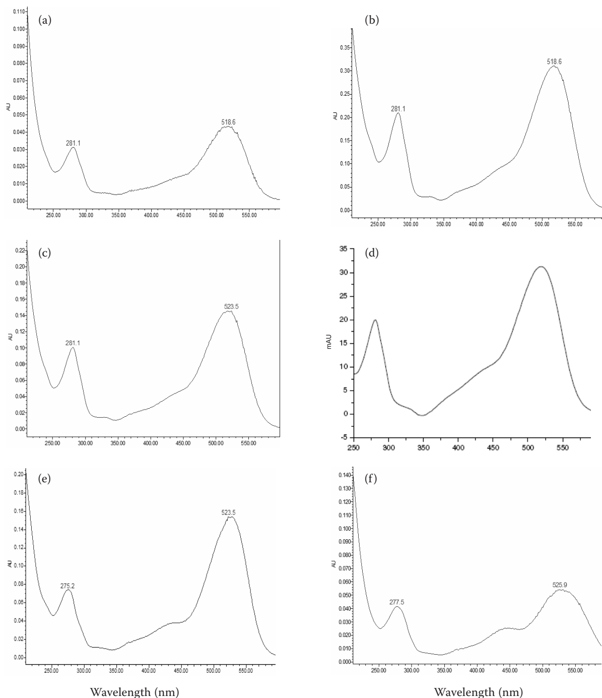
Figure 5. UV-Visible spectrum of peaks 1–5 recoded with a photodiode array detector (PAD) from 200 nm to 600 nm: (a) peak 1; (b) peak 2; (c) peak 3; (d) standard cyanidin 3- O -glucoside (Cy-3-Glu); (e) peak 4; (f) peak 5
