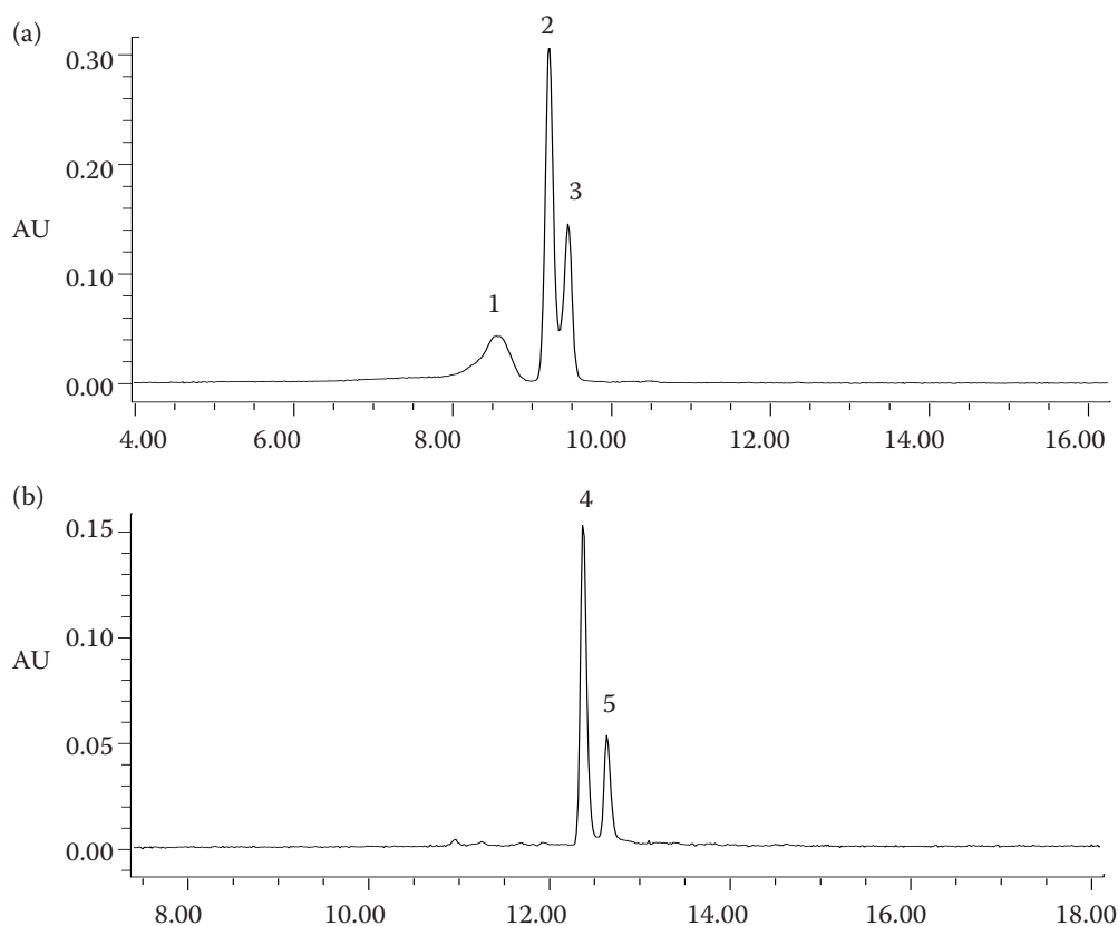
Figure 2. HPLC-PAD chromatogram recorded at 520 nm corresponding to (a) the purified extract from the fruit of waxberry; (b) the purified extract from the pigment of waxberry after acid hydrolysis
