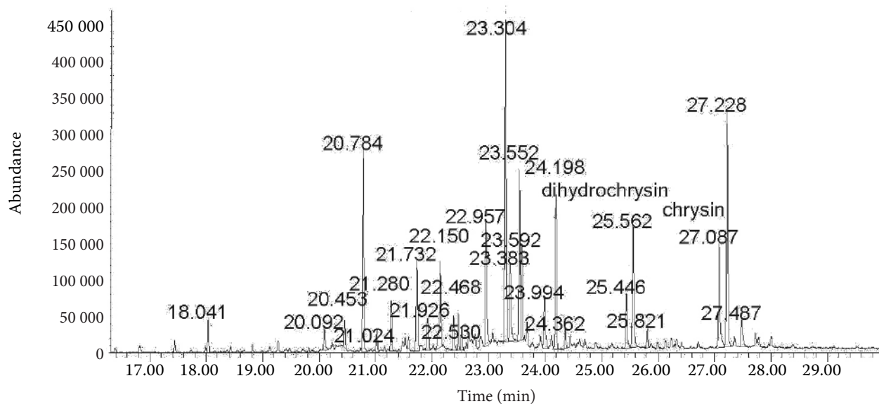
Figure 4. GC-MS chromatogram of the fraction 4 obtained from honey mixed samples by preparative HPLC-UV-VIS
