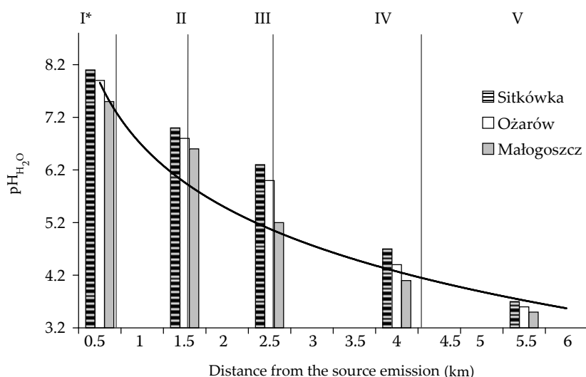
Fig. 2. Change of modal value of pH H 2 O of bark at the three alkalyzed stands close to the cement plants at Sitkówka, Ożarów, Małogoszcz
