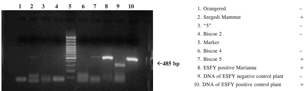
Figure 1. ESFY detection by nested PCR. Products of amplification were separated in 1.5% agarose gel
