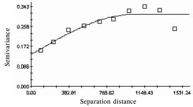
Figure 4. pH data set empirical variogram and fitted model; the fitted spherical model has parameters: a nugget effect of 0.136, range 1037 m; r^2 = 0.817 and RSS-residual sums of squares of 3663 (the lowest of all models)
