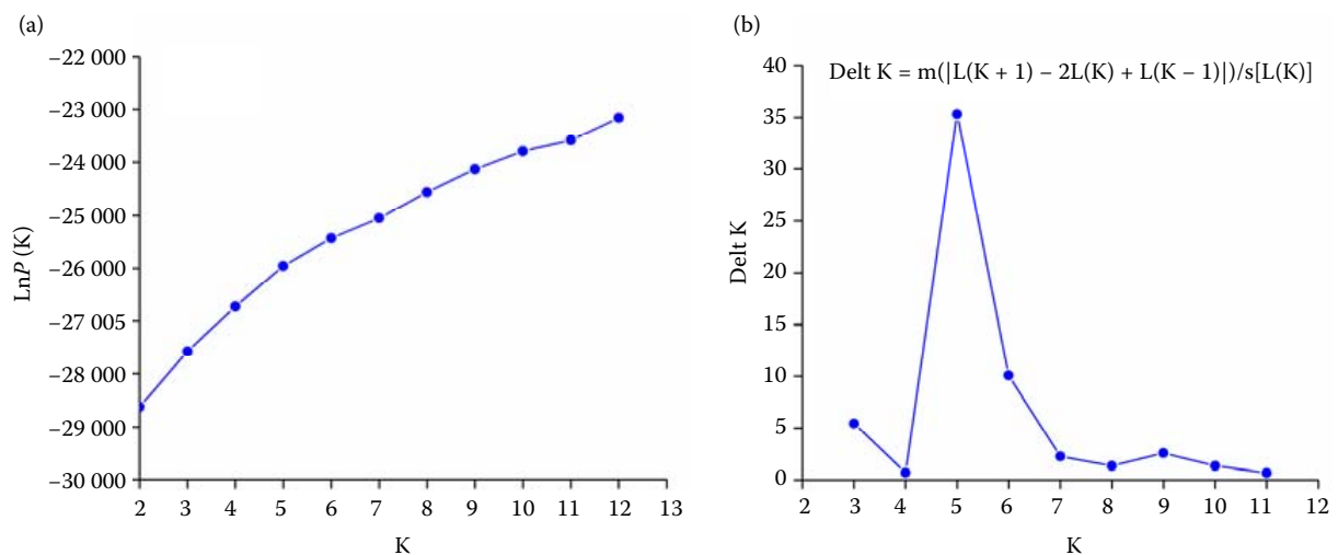
Figure S2. STRUCTURE estimation of the mapping panel: (a) evolution of the natural logarithm probability of the data against K; (b) magnitude of Delt K for each K value
