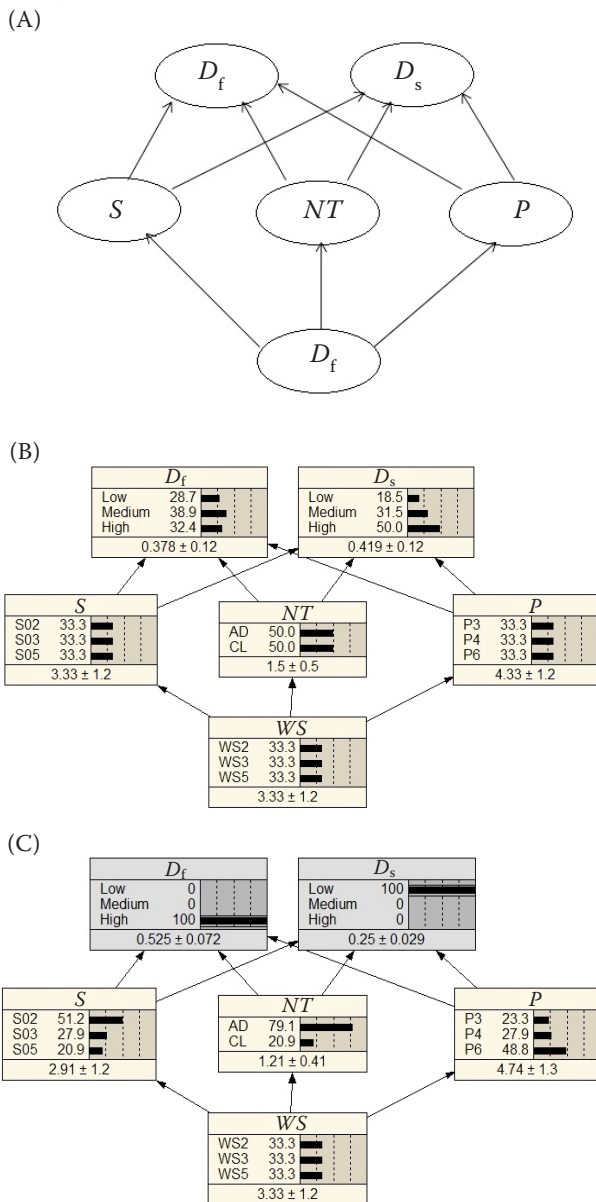
Figure 4. Application of Bayesian network for the analysis of deposits on leaves and soil deposition (A) Bayesian network structure considered, (B) the model after parameter learning in Netica and (C) prediction of the model when the evidence variables are deposits on th foliage ( D_f ) and deposits on the soil ( D_s )
