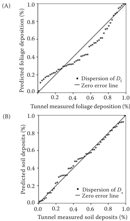
Figure 2. Comparison of models findings with tunnel measured data (A) foliage deposition ( D_f ) and (B) soil deposits ( D_s )
