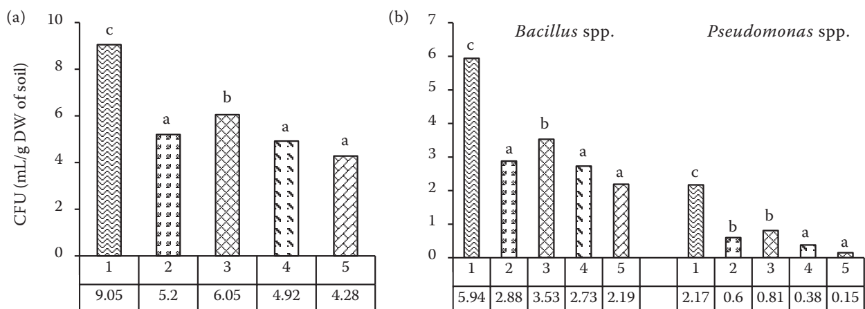
Figure 1. Total number of (a) bacteria and (b) Bacillus spp. and Pseudomonas spp. isolated from the soil of particular experimental treatment (means from the years 2010–2012). 1 – soil after rye cultivation; 2 – soil after buckwheat cultivation; 3 – soil after white mustard cultivation; 4 – soil after sunflower cultivation; 5 – soil without cover crops cultivation. Means differ significantly ( P < 0.05 ) if they are not marked with the same letter. CFU – colony forming units; DW – dry weight
