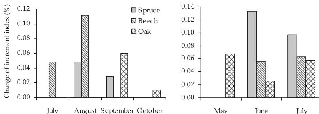
Fig. 5. The intensity of the effect of monthly precipitation during the vegetation period of the previous year (left) and of the actual year (right) on increment indexes of tree species
