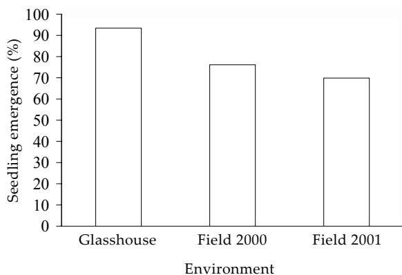
Figure 1. Comparison of environments for seedling emergence percentage (* means with different letter are significant at 0.05 significance level, LSD_{0.05} = 0.362 )
