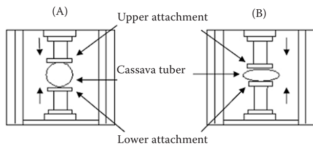
Figure 1. Compression of the TME 419 variety of cassava tuber in the (A) longitudinal and (B) transverse loading orientations using the universal testing machine
