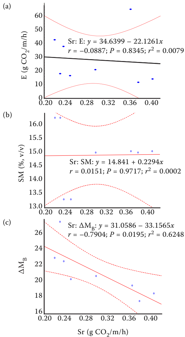
Figure 2. The simple regression analysis on soil respiration (Sr) and (a) evapotranspiration (E); (b) soil moisture (SM) and (c) changes in soil moisture ( \Delta M_B )
