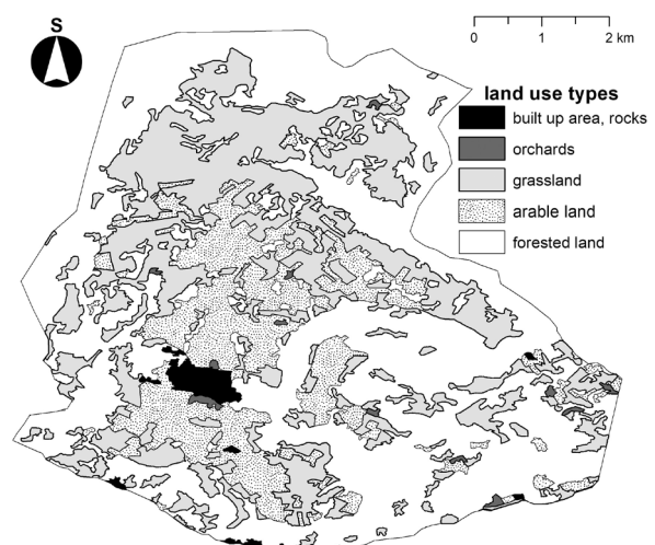
Figure 3. Land use map of the study area
