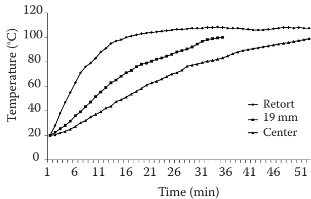
Figure 1. Temperature rise in two points inside 73 mm x 103 mm cans filled with motabbal al-bathinjan during processing in still steam retort
