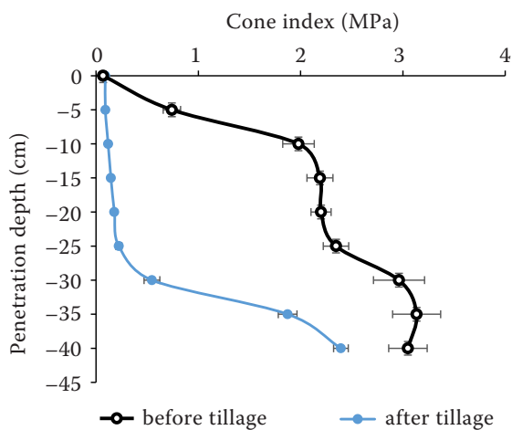
Figure 2. Results of the penetrometer tests on the bin soil before and after tillage
