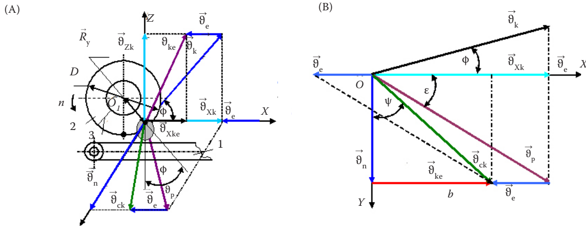
Figure 2. (A) Circuit design and (B) plan of the velocity of the oblique impact of the root with the working surfaces of the combined cleaning system
