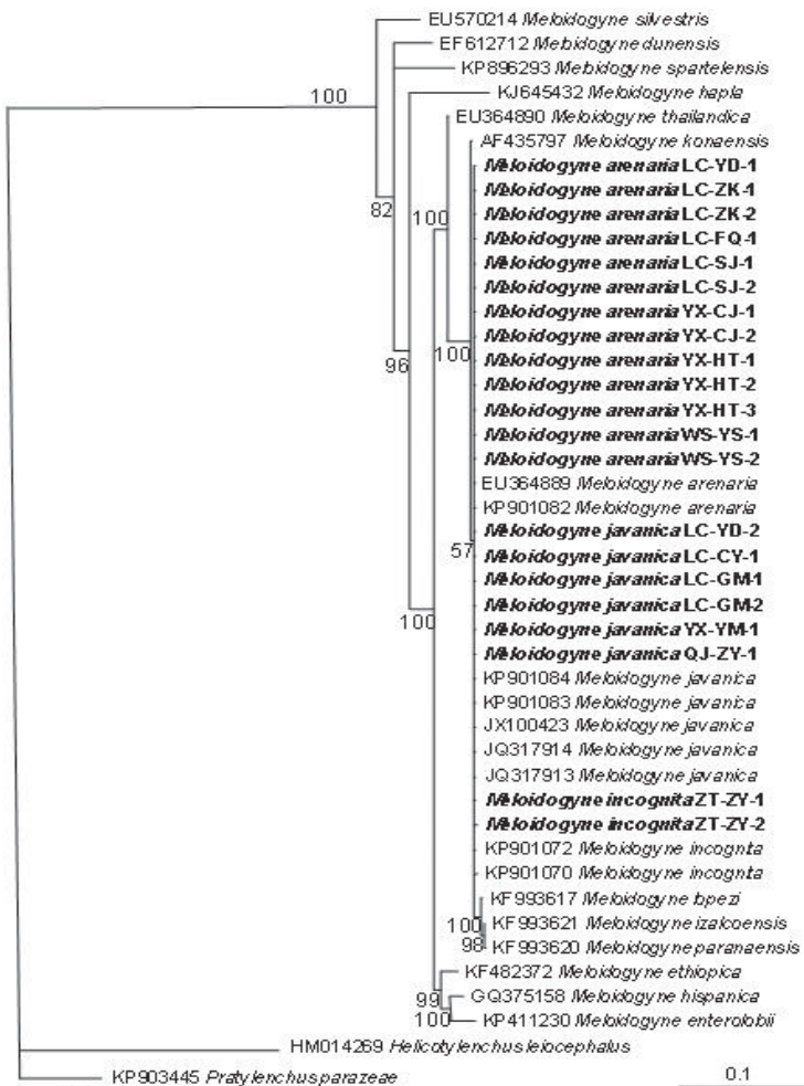
Figure 2. The 10001st Bayesian consensus tree inferred from 28S D2-D3 under GTR+G model –lnL = 2812.7192; AIC = 5643.4385; freqA = 0.2050; freqC = 0.2134; freqG = 0.3170; freqT = 0.2646; R(a) = 0.3968; R(b) = 2.1167; R(c) = 1.1724; R(d) = 0.2998; R(e) = 3.0376; R(f) = 1.0000; Pinvar = 0.0000; Shape = 0.9882; posterior probability values exceeding 50% are given on appropriate clades
